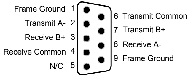
Back (Solder-side) View
