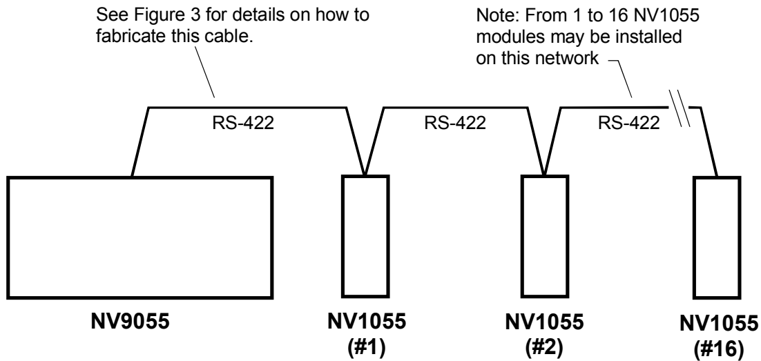
Figure 5 - Connecting NV1055 Mix/Minus with Router Modules to an NVISION NV9055 Remote Control Panel
